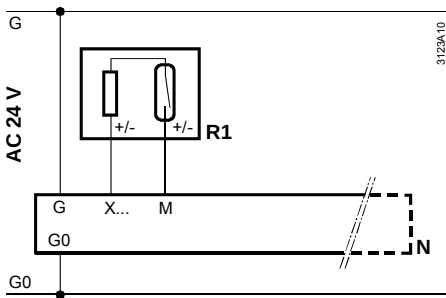
Diagram 3: Measuring section with pulse source
