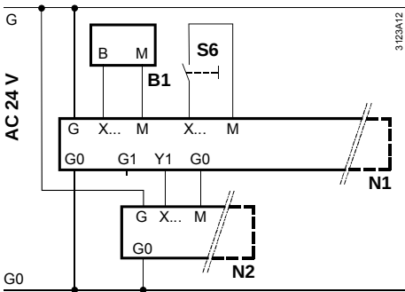
Diagram 4: Multiple use of sensors (B1, N2), external changeover of operating mode (S6)
