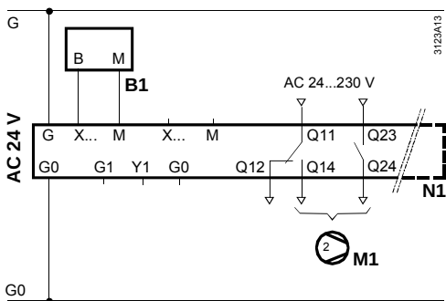
Diagram 5: Connection of a 2-speed fan
