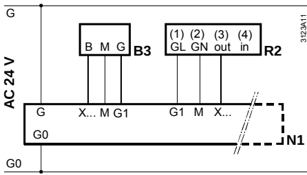
Diagram 2: Measuring section with active sensor and signal source
