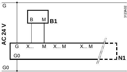
Diagram 1: Measuring section with passive sensor
